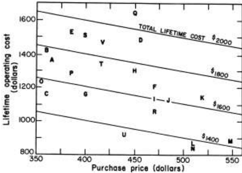
Figure 2 Scatter plot and cost data on 22 1976 refrigerators. The scatter plot (and Table on page 47) show little correlation between purchase price and efficiency. Source: Goldstein & Rosenfeld (13).
