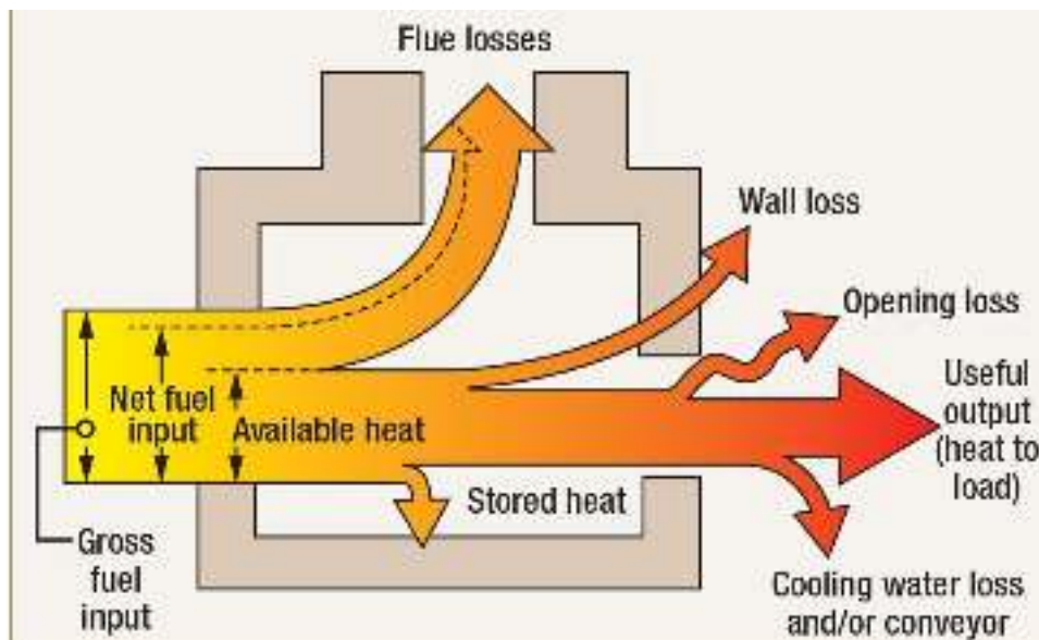
Figure 70: Furnace losses
