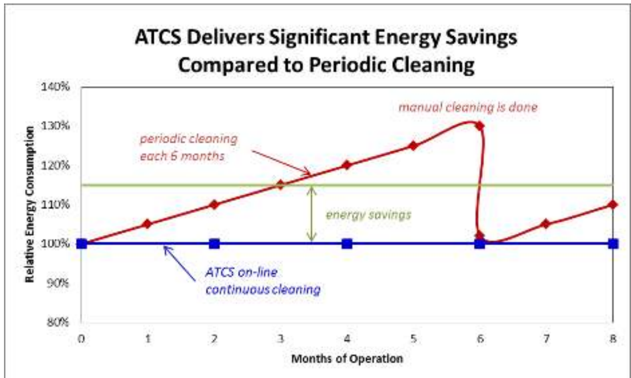
Figure 38: Benefit of automatic tube cleaning system (Source: Trane)
