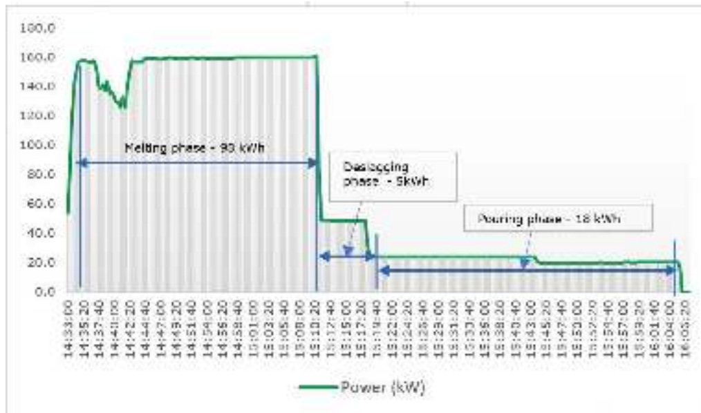
Figure 67: Different phases of induction furnace batch process – an example (Source: STENUM Asia)
