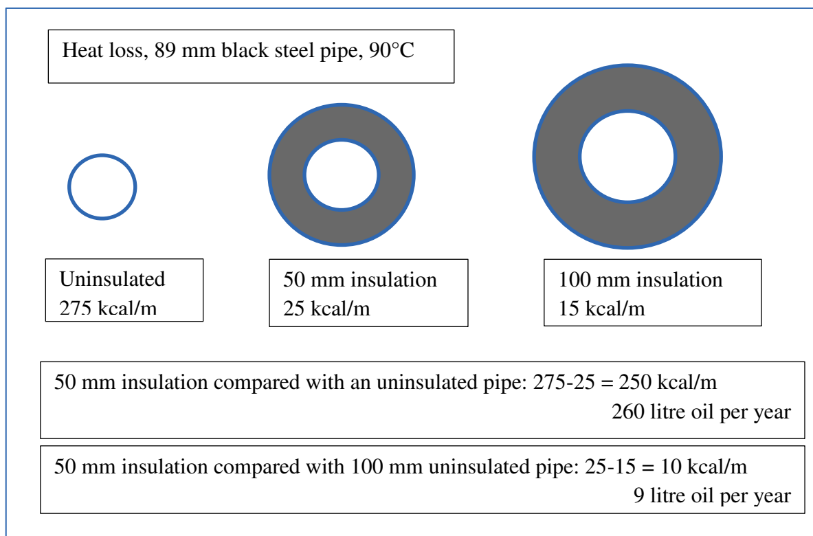
Figure 89: Illustration of optimal insulation
