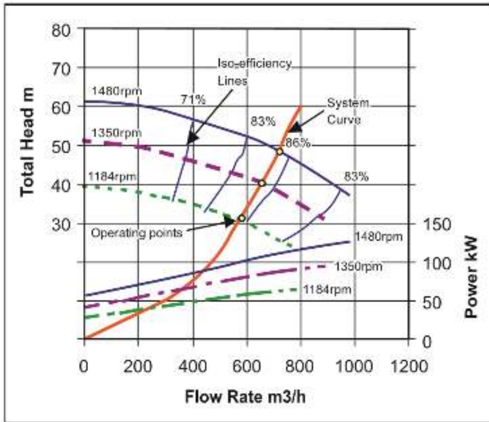
Figure 55: Effect of speed change in a system with no static head
