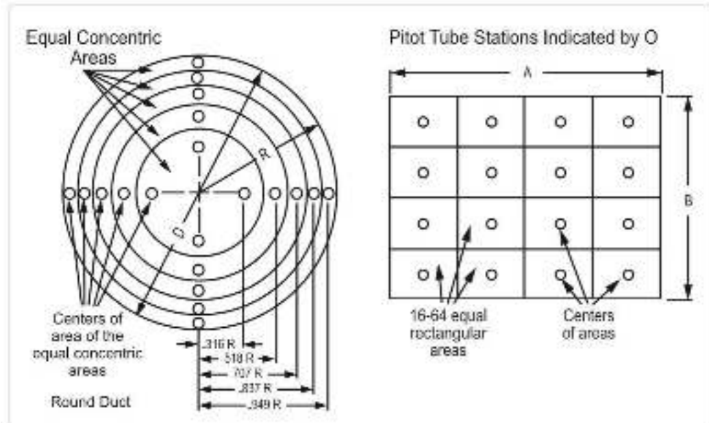
Figure 43: Traverse on round and square duct areas
