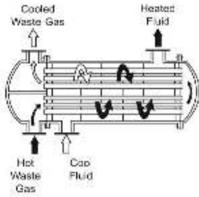
Figure 85: Tube type recuperator
