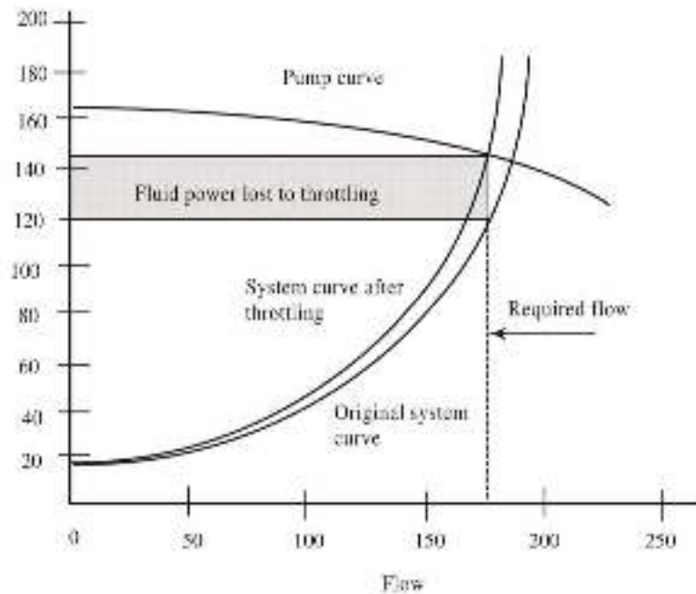
Figure 53: Before impeller trimming
