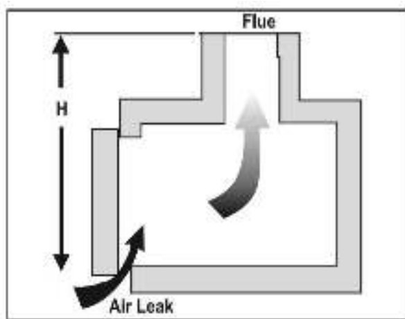
Figure 73: Air infiltration in furnace
