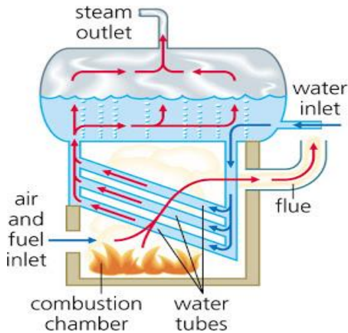
Figure 63: Water tube boiler (Source: BEE)
