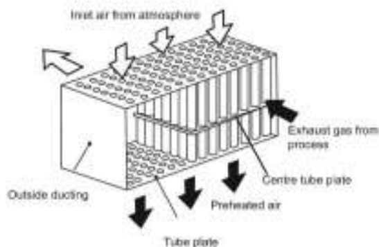
Figure 83: Recuperator configuration
