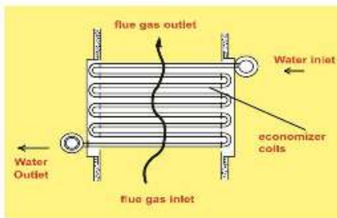
Figure 87: Economiser
