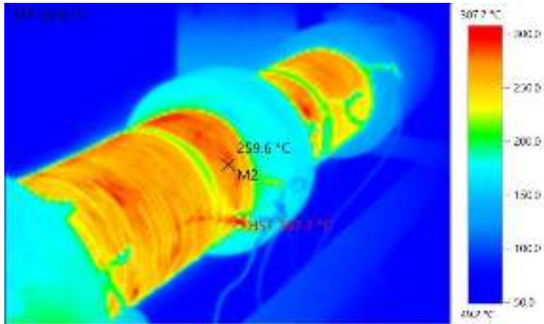
Figure 88: An example of thermal image taken from thermal camera
