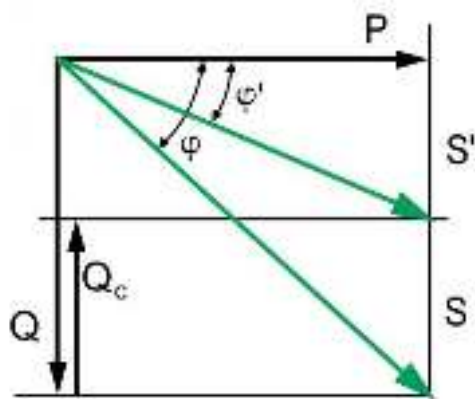
Figure 16: Power factor correction triangle
