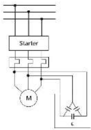
Figure 25: Method 1- Capacitor is connected directly to the motor
