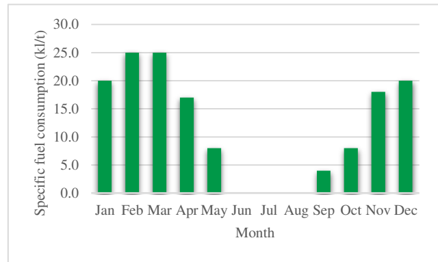
Figure 4: Historical fuel intensity pattern for a spinning mill
