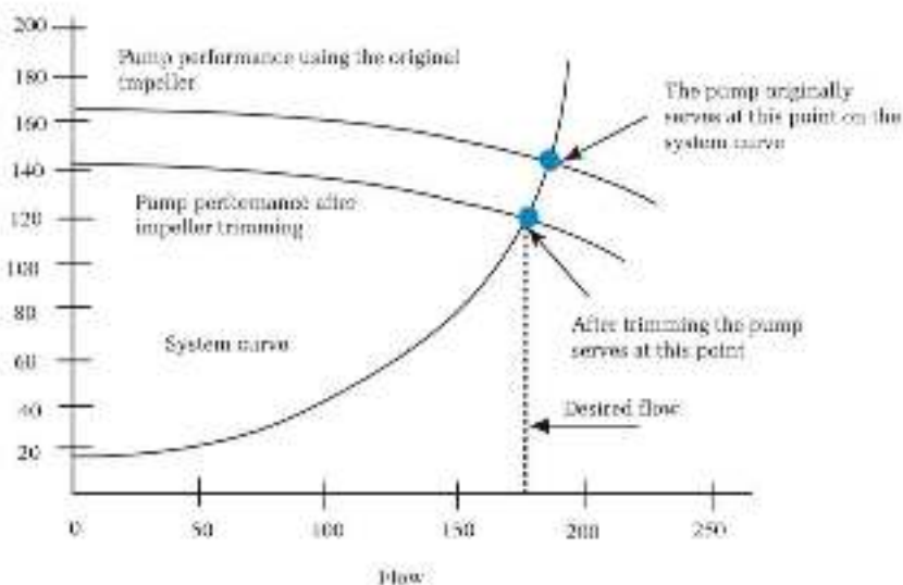
Figure 54: After impeller trimming
