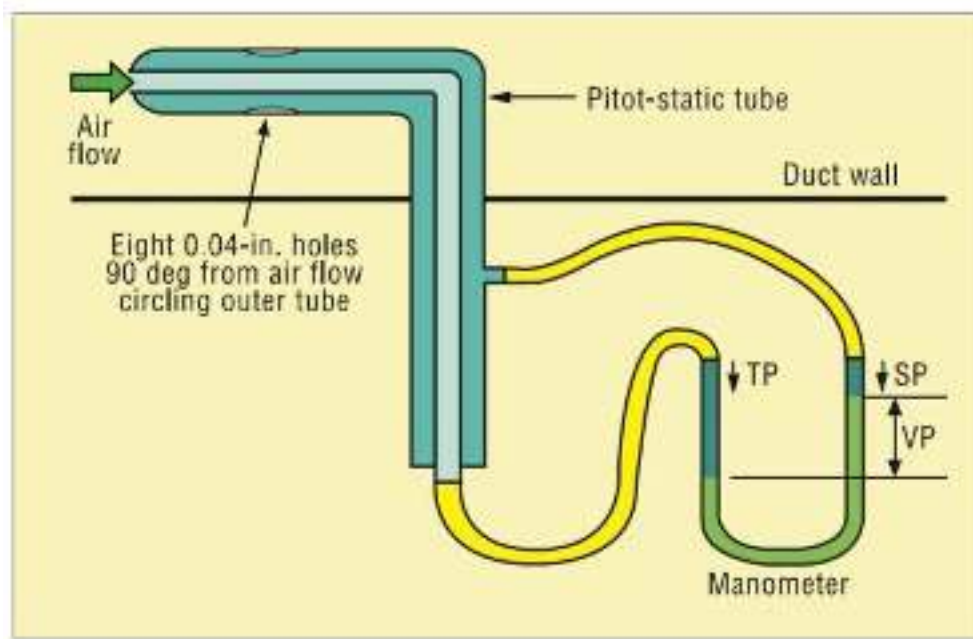
Figure 42: Measurement by pitot tube
