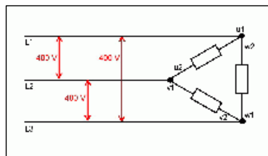
Figure 24: Delta connection
