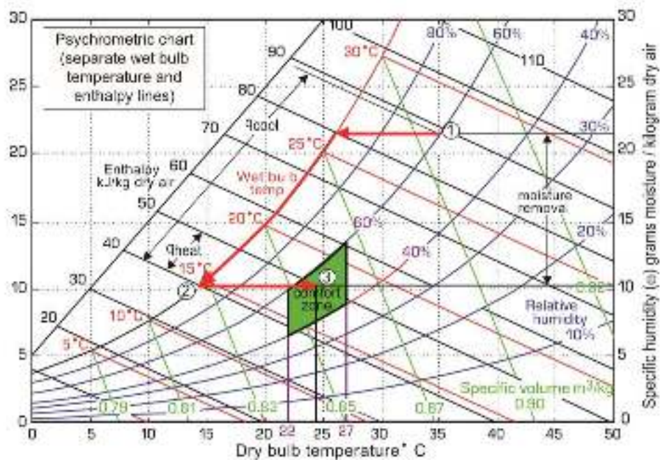
Figure 36: Psychrometric chart depicting human comfort zone (Source: BEE)
