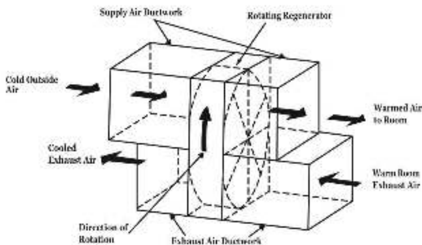
Figure 86: Sketch of heat wheel
