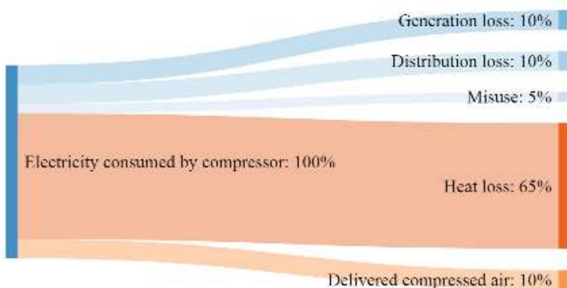
Figure 31: Sankey diagram of compressed air losses
