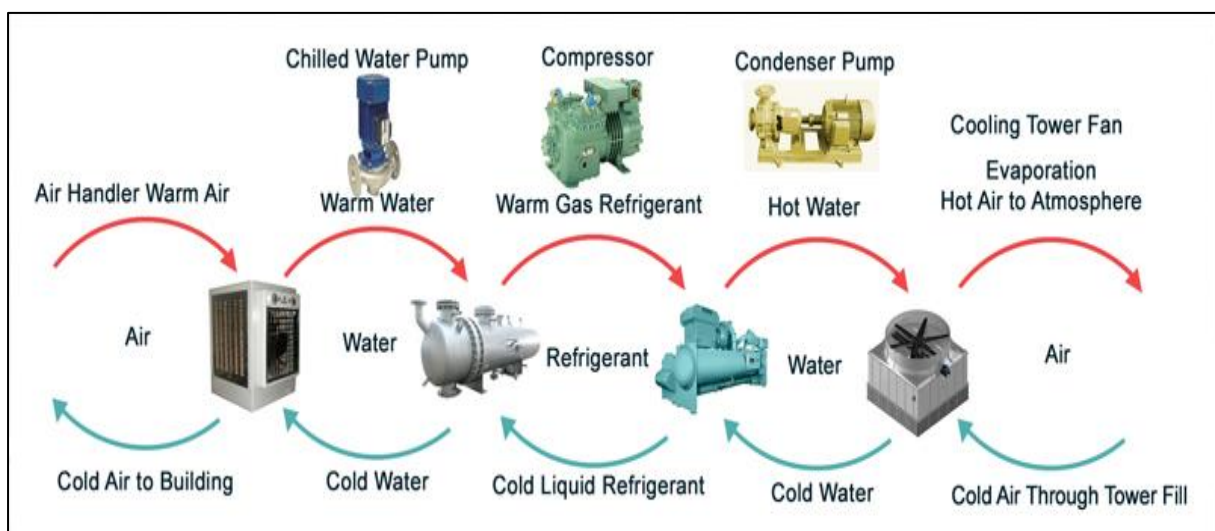
Figure 34: Heat Transfer Loops in refrigeration system
