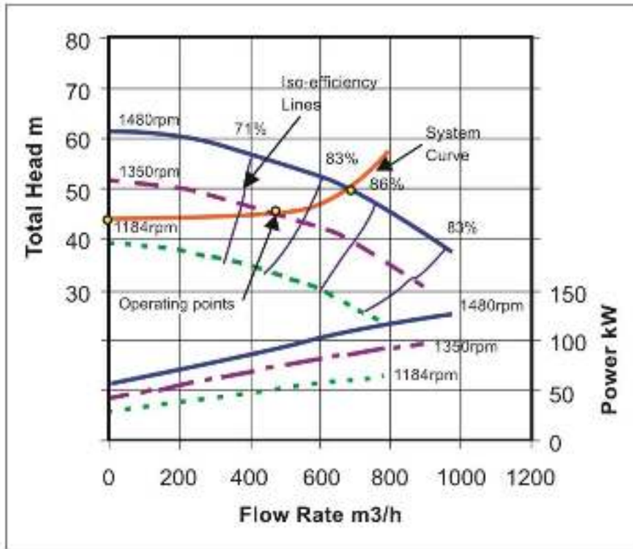
Figure 56: Effect of speed change in a system with high static head
