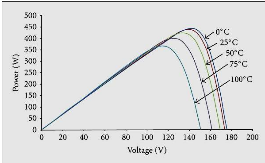
Figure 95: Effect of temperature change on power and voltage
