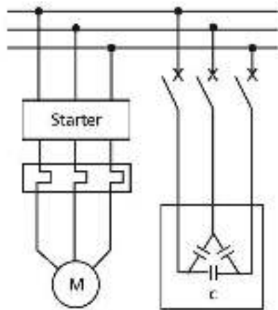
Figure 26: Method 2 - Capacitor is connected to the motor before starter
