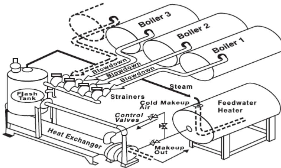
Figure 66: Blowdown heat recovery system
