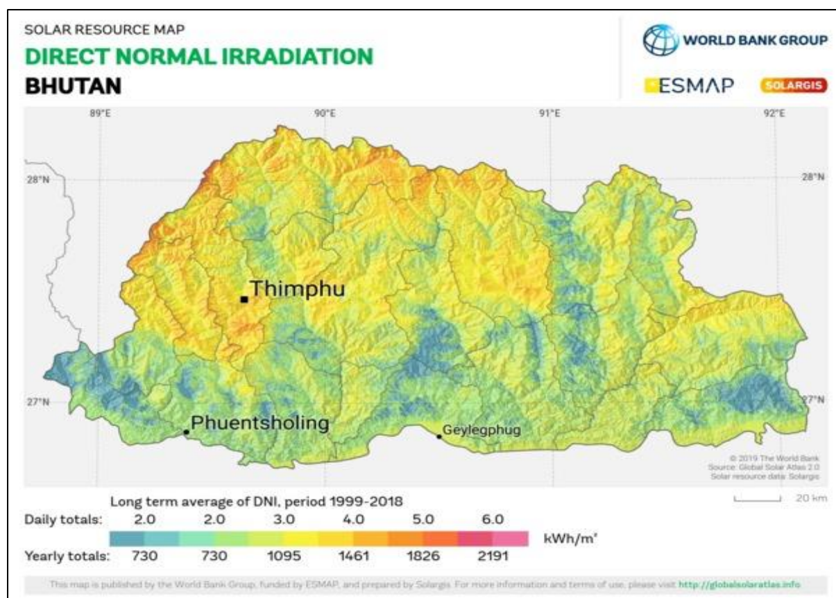
Figure 93: Direct Normal Irradiation map of Bhutan (Source: World bank group)
