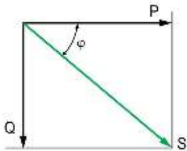
Figure 13: Power triangle
