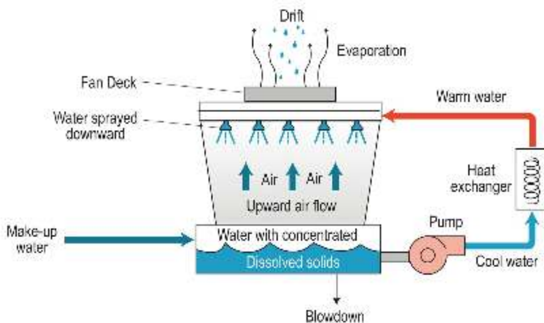
Figure 59: Cooling tower with closed loop
