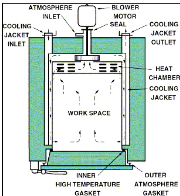
Figure 82: Typical industrial oven
