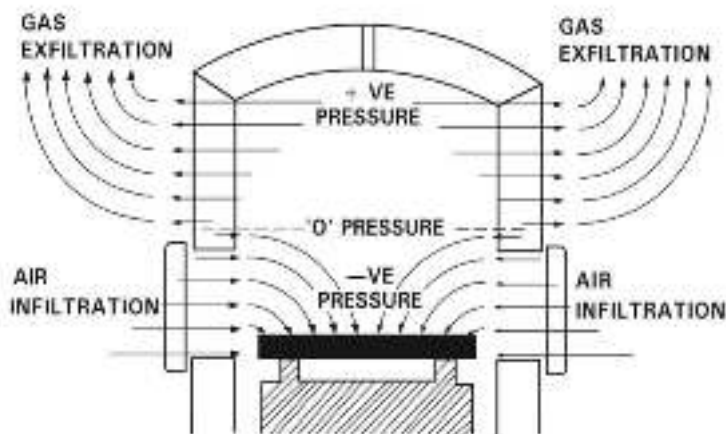
Figure 78: Effect of pressure on the location of zero level and infiltration of air (Source: BEE)
