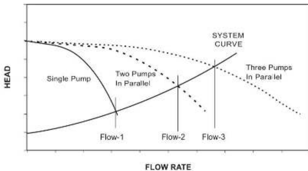
Figure 58: Typical head-flow curve for pumps in parallel operation
