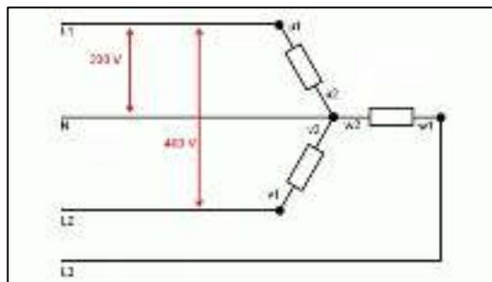
Figure 23: Star connection
