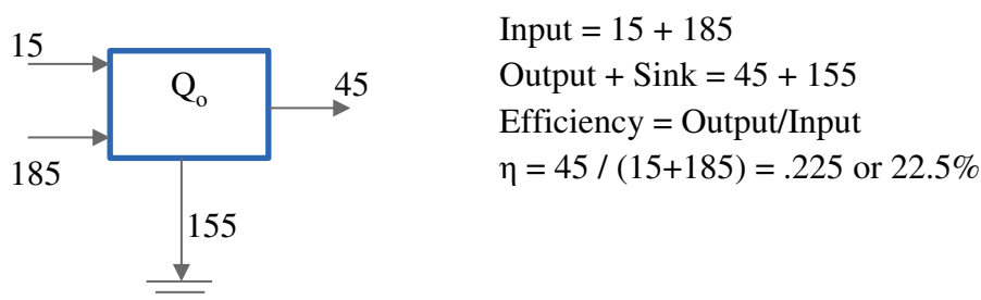
Figure 100: Efficiency and losses
