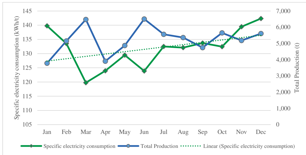
Figure 6: An example of line graph depicting specific electricity consumption (SEC) over time and increasing trend of SEC
