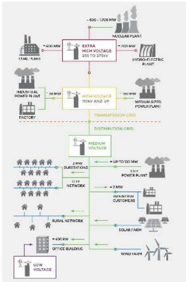
Figure 10: Illustration of electricity transmission and distribution system (Source: UNEP)
