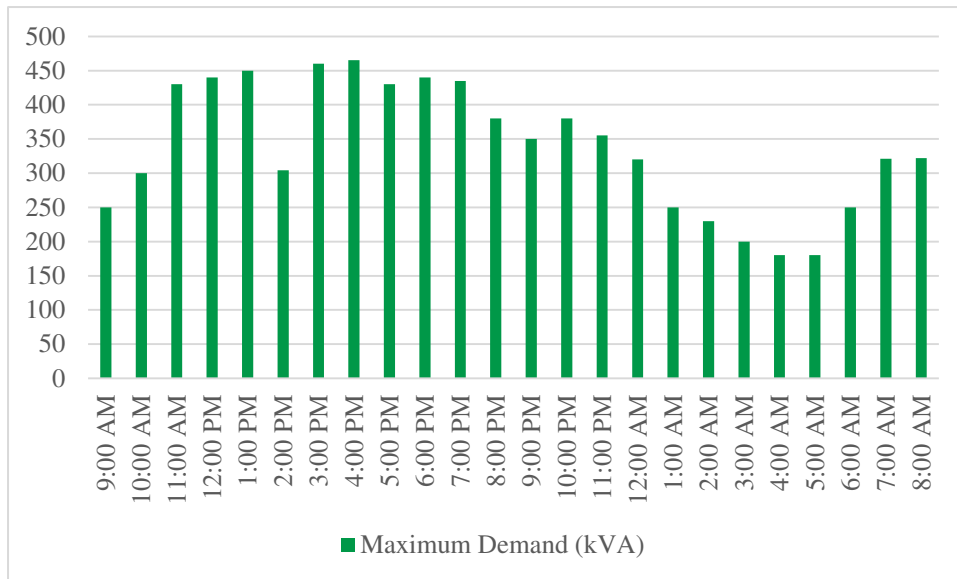
Figure 11: Hourly load curve
