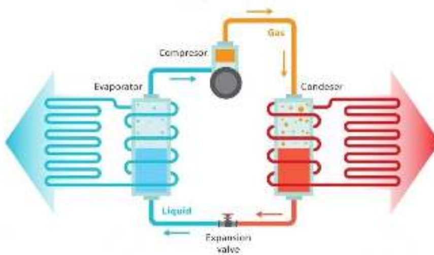
Figure 37: Vapour compression refrigeration system
