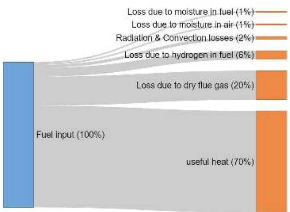
Figure 101: Sankey diagram for Boiler fuel input to heat output
