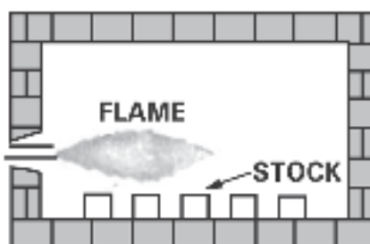
Figure 77: Correct alignment of burners
