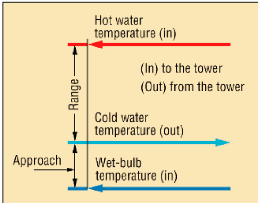
Figure 61: Range and Approach
