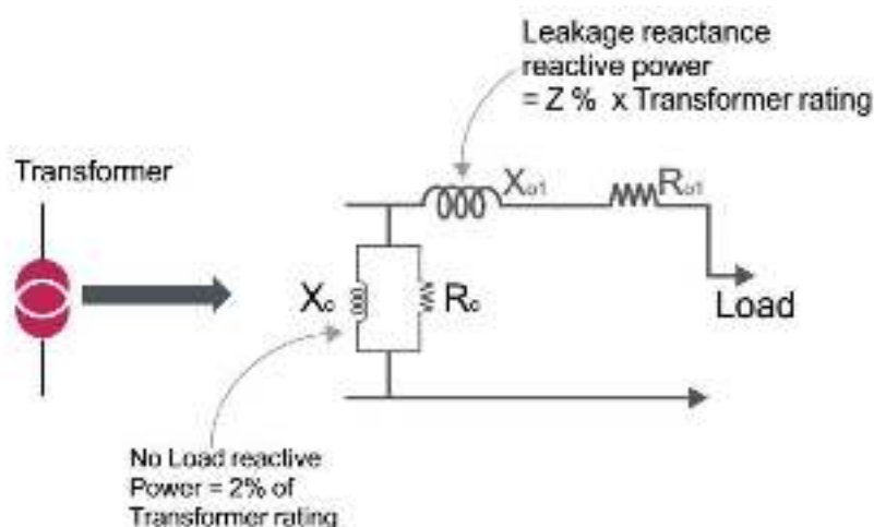
Figure 15: No-load compensation for transformer
