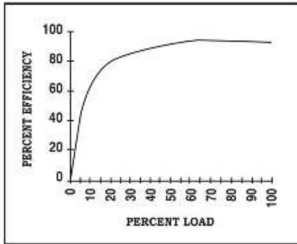
Figure 22: Effect of motor loading on efficiency (Source: BEE)
