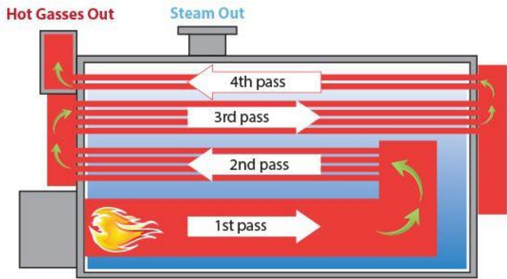
Figure 62: Fire tube boiler
