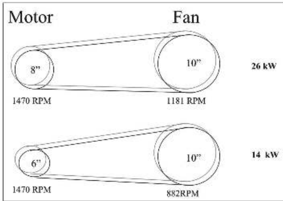
Figure 44: Pulley change
