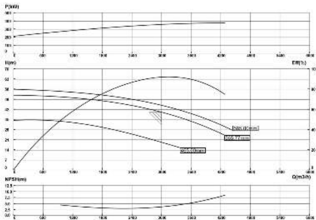
Figure 51: Typical pump curve provided by manufacturer
