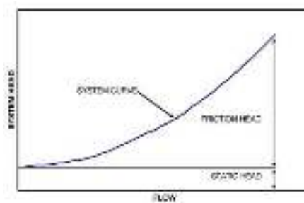
Figure 49 System head with low static head
