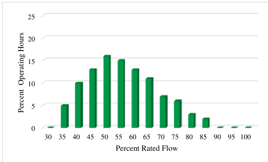
Figure 29: Example of an excellent variable speed drive candidate
