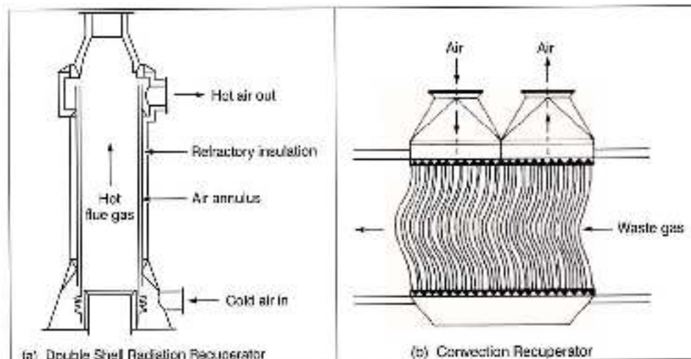
Figure 79: Recuperators
