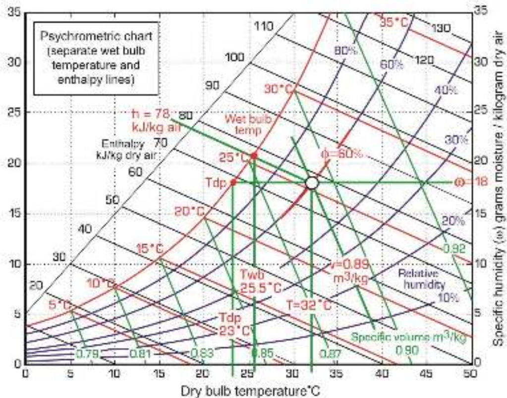
Figure 35: Psychrometric chart (Source: BEE)
