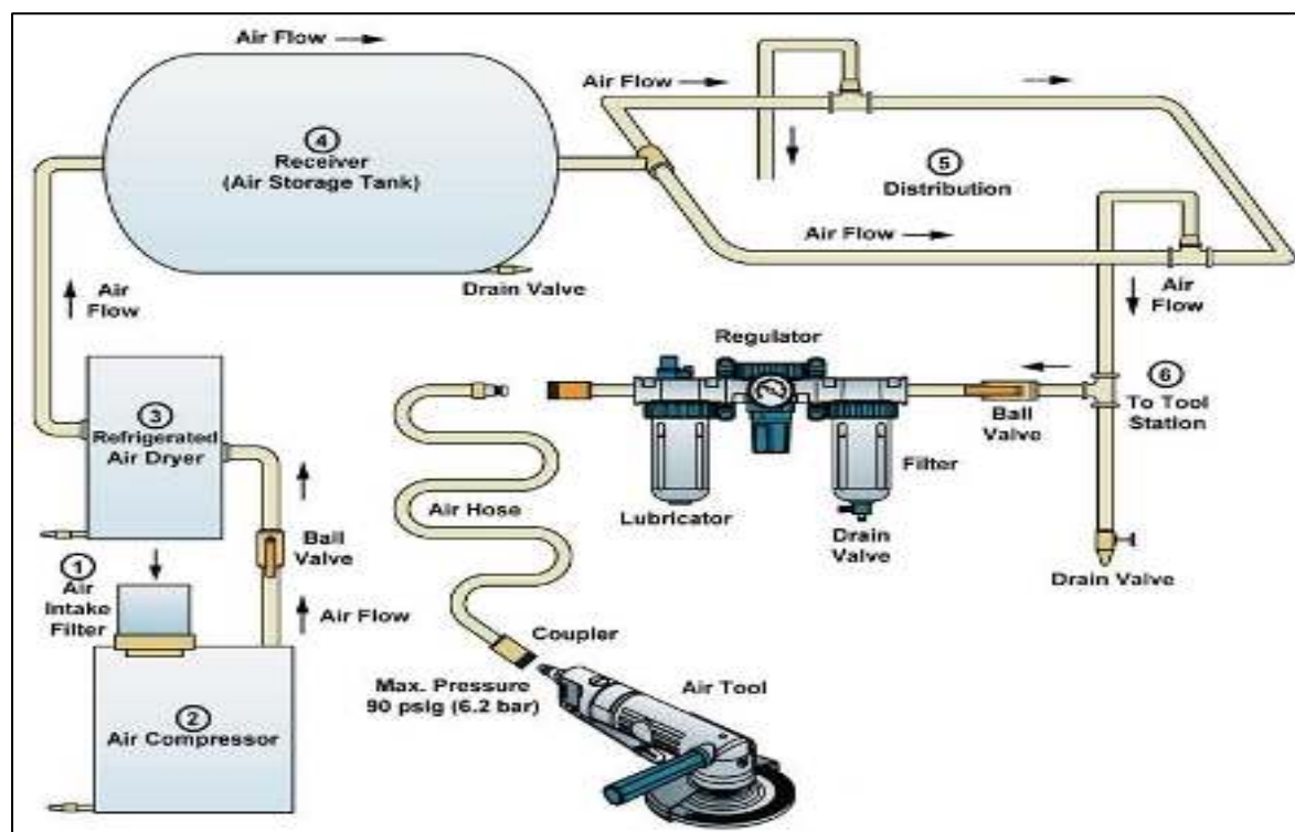
Figure 33: Figure of elements of compressed air system showing generation, distribution, and usage (Source: Gison Pneumatics)
