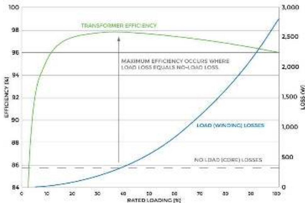
Figure 18: Transformer losses as a percentage (%) of load (Source: UNEP)
