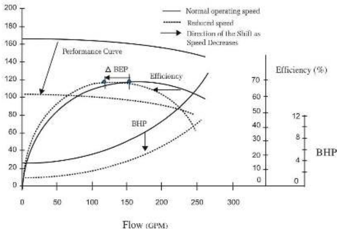
Figure 57: Effect of VFD
