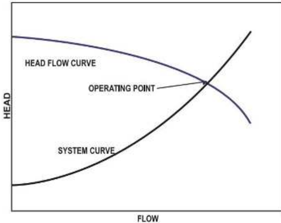
Figure 52: Pump operating point
