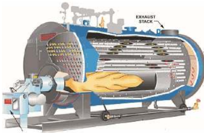
Figure 64: Packaged Boiler (Source: BEE)
