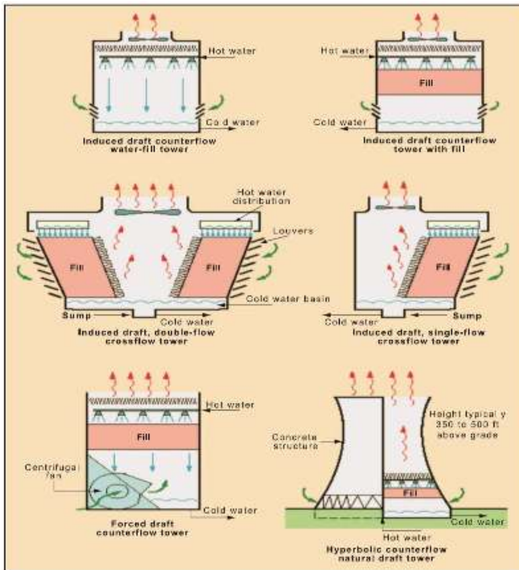
Figure 60: Types of cooling tower (Source: BEE)
