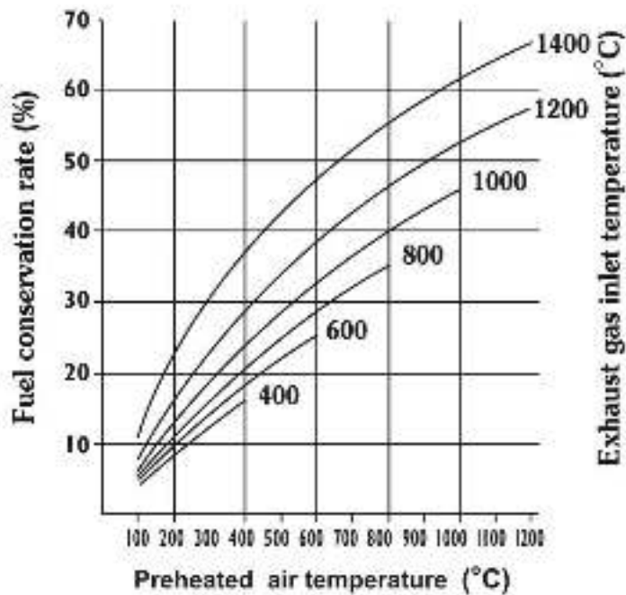
Figure 80: Fuel savings rate by preheated air temperature (Source: BEE)
