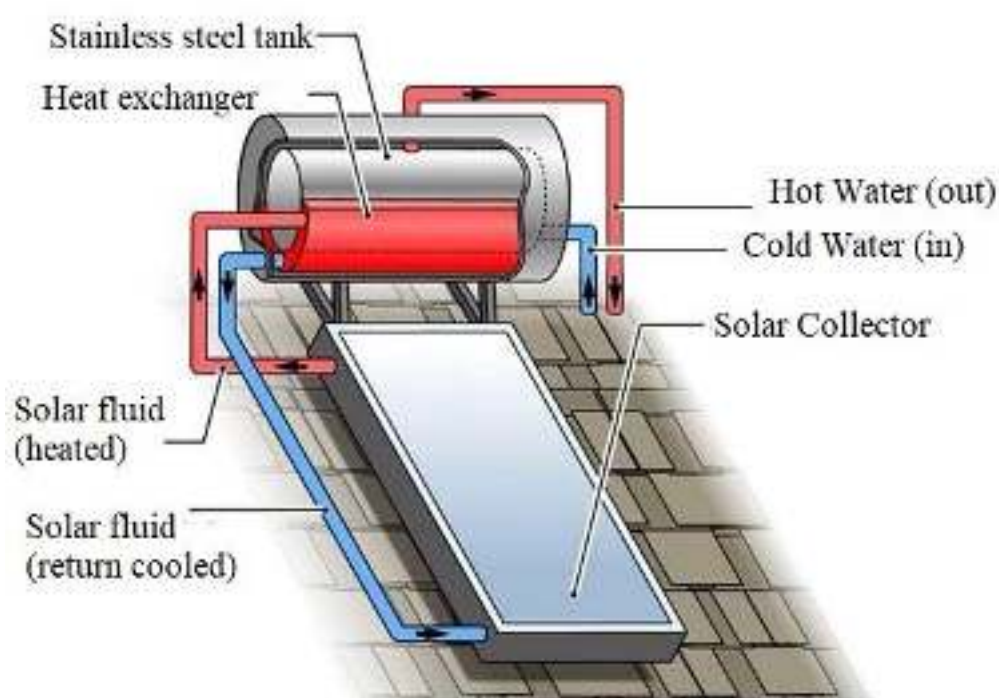
Figure 96: Solar water heater
