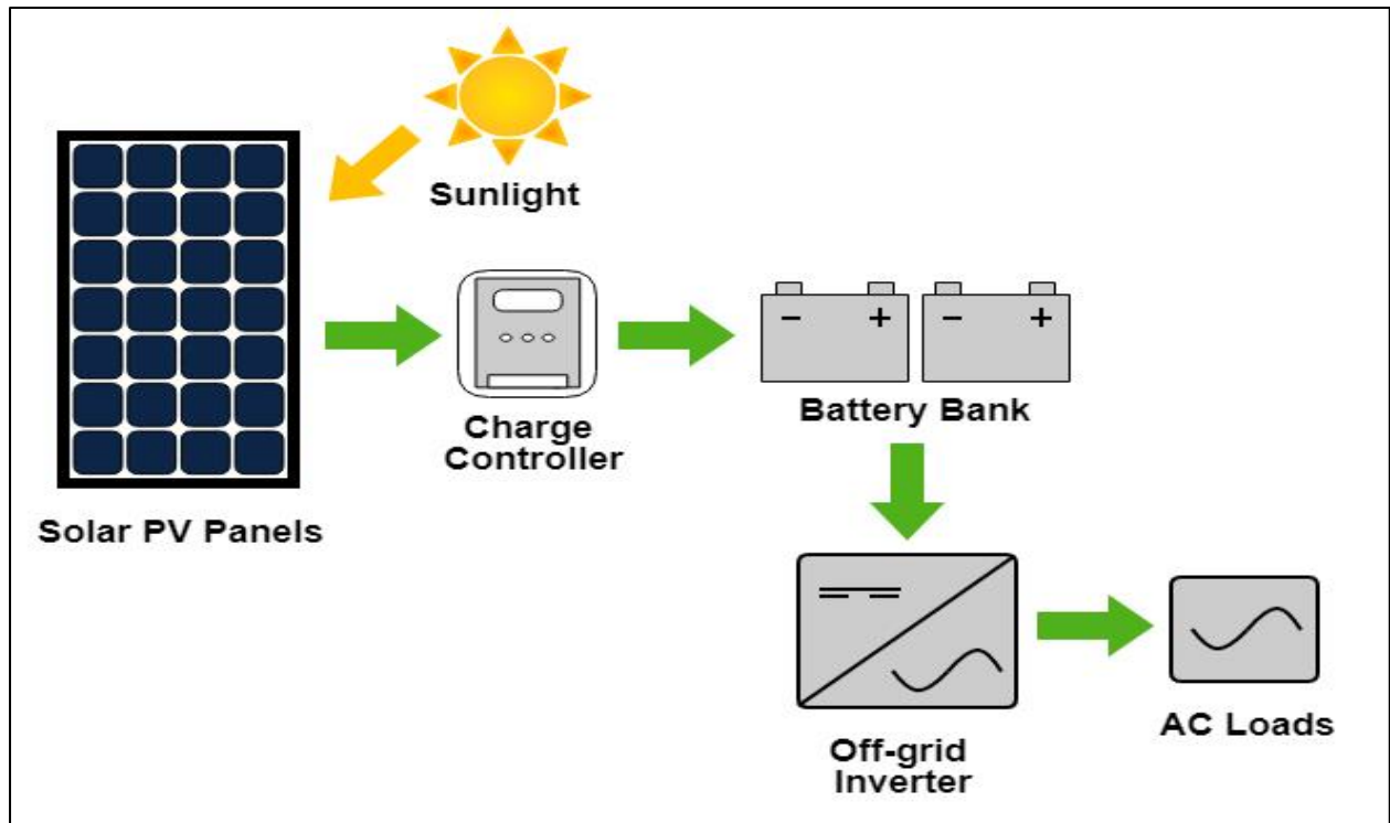
Figure 92: Stand-alone PV system (Source: Apricus solar)
