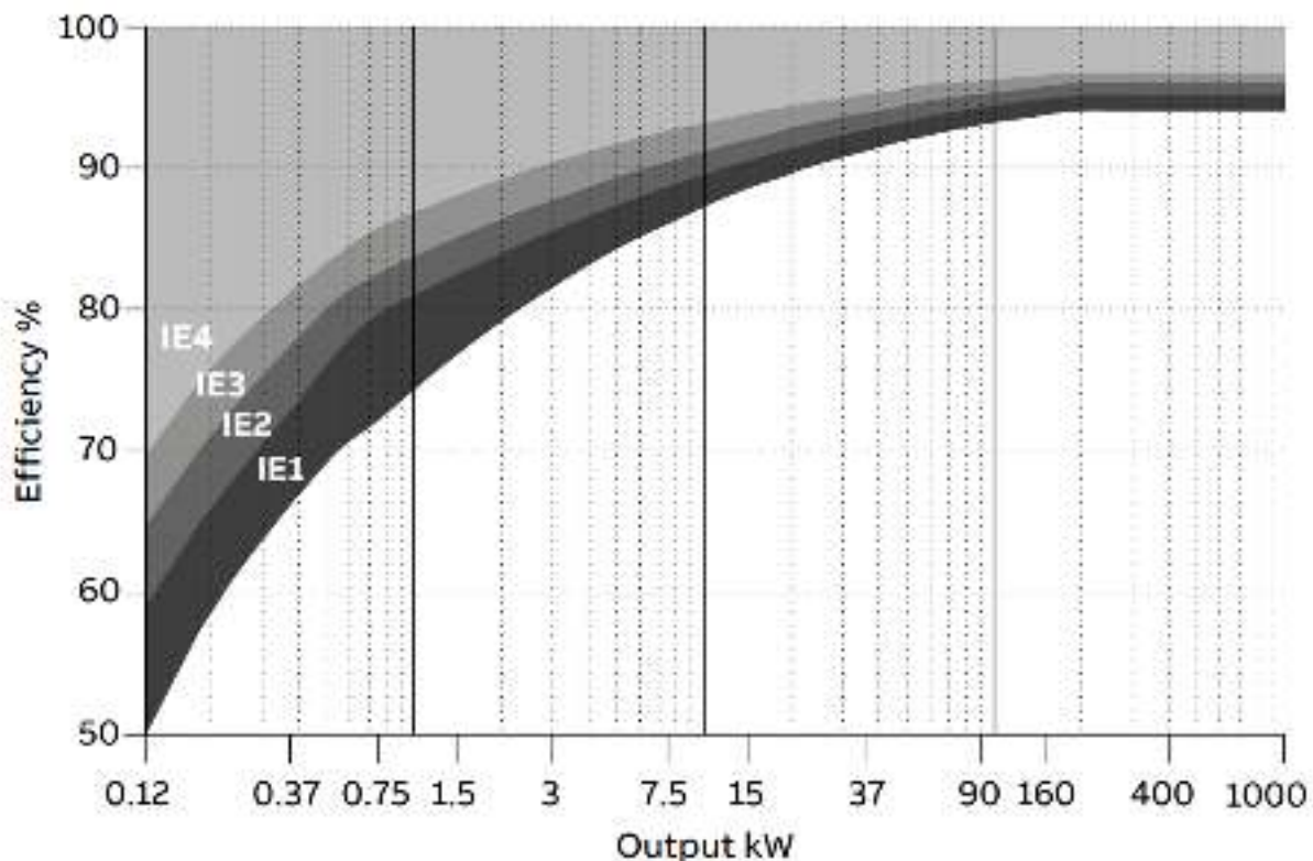
Figure 27: IE efficiency classes for 4 pole motors at 50 Hz (Source: ABB)
