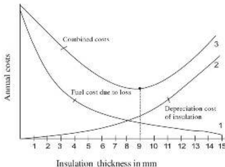
Figure 90: Determination of economic thickness of insulation (Source: BEE)
