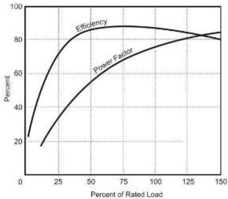
Figure 20: Effect of motor loading on efficiency & power factor (Source: BEE)
