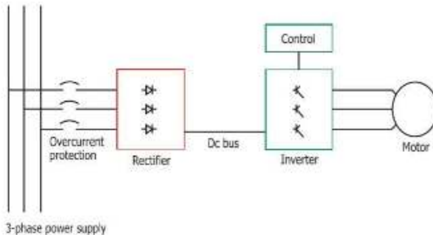
Figure 28: Component of VFD system
