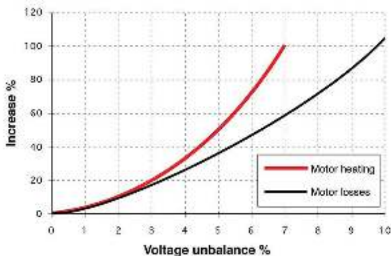
Figure 19: Voltage unbalance (%) versus motor losses & motor heating (Source: BEE)
