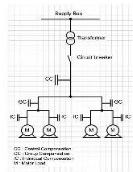
Figure 17: Different compensation modes for power factor improvement
