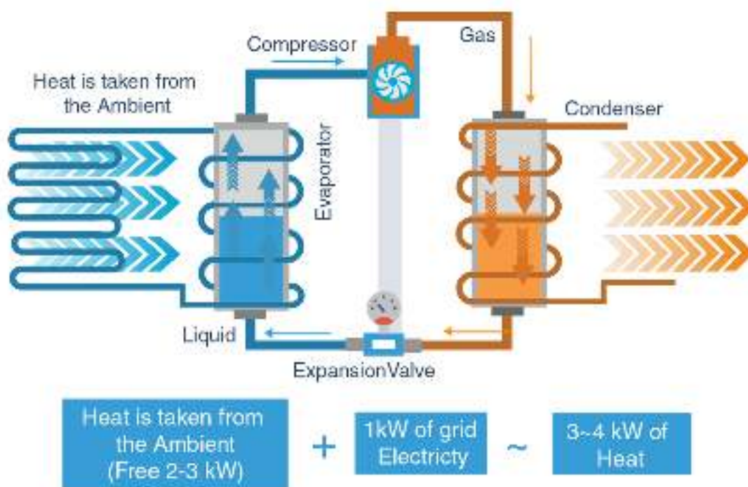
Figure 40: Heat Pump working (Source: Aspiration energy)
