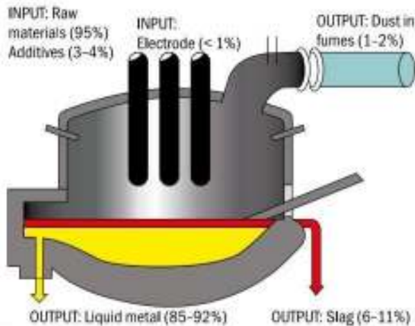
Figure 69: Material balance of EAF
