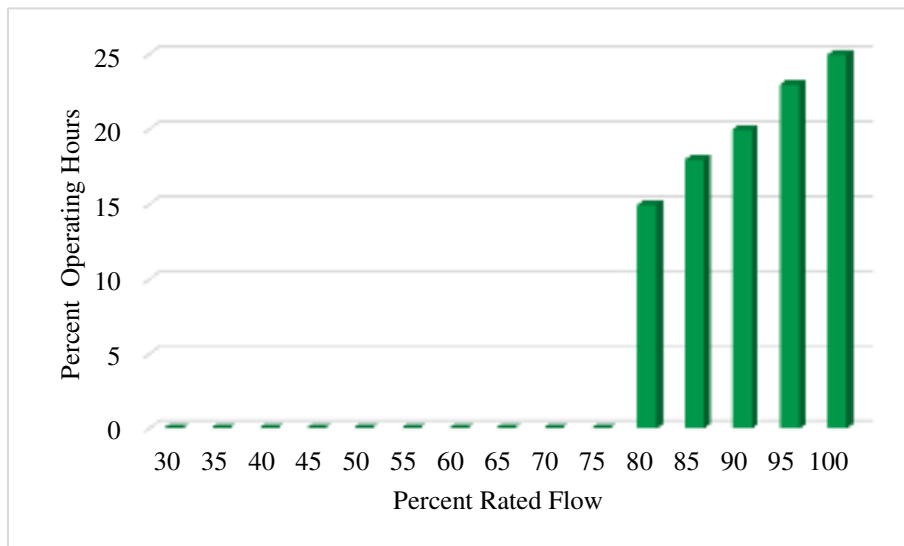
Figure 30: Example of a poor variable speed drive candidate
