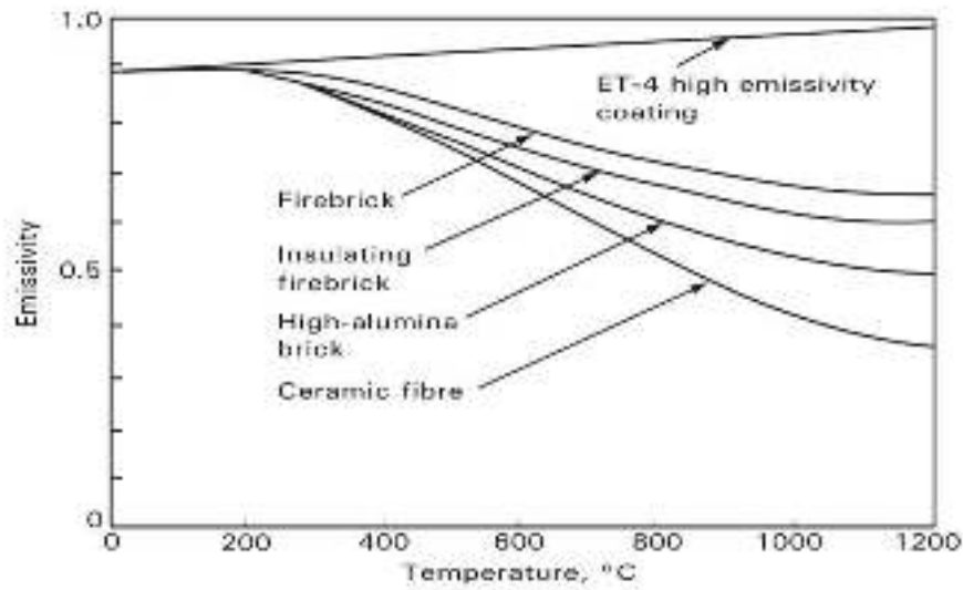
Figure 91: High emissivity coatings of various insulating materials
