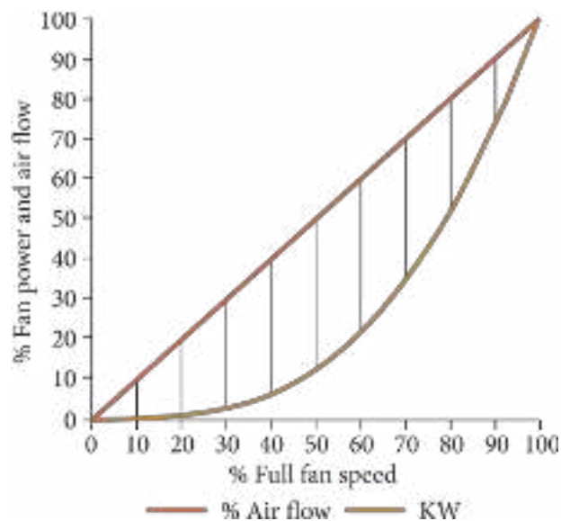
Figure 39: Effect of speed on power and air volume
