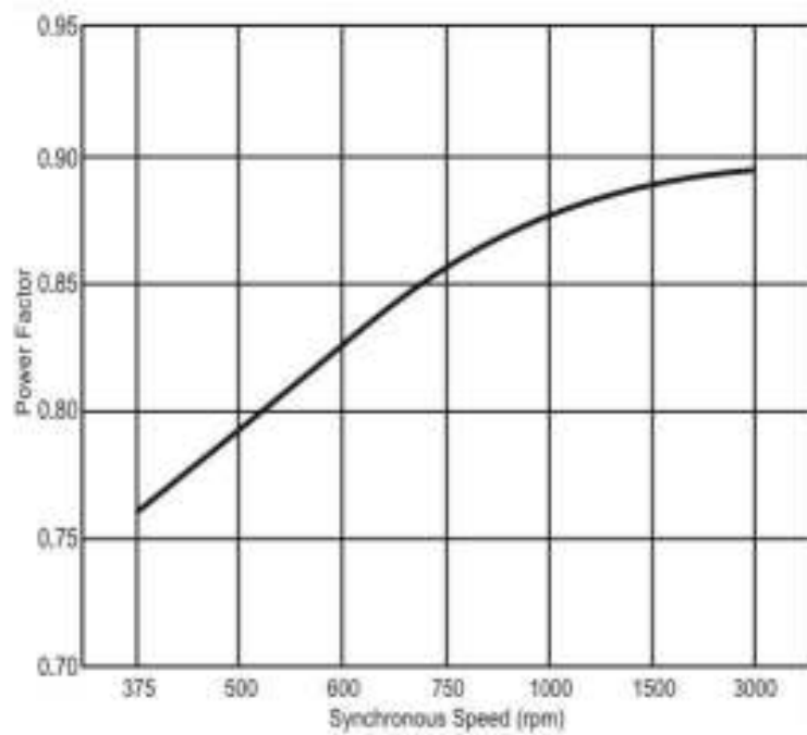
Figure 21: Effect of motor speed on power factor (Source: BEE)
