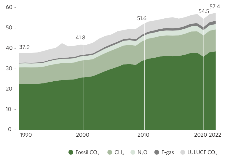
Total net anthropogenic greenhouse gas emissions, 1990–2022 (gigatons of CO 2 equivalent)
