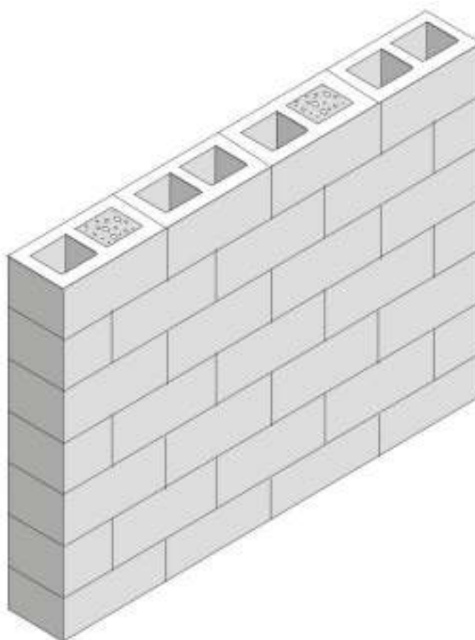
Figure 4.3.5 – Masonry Wall
