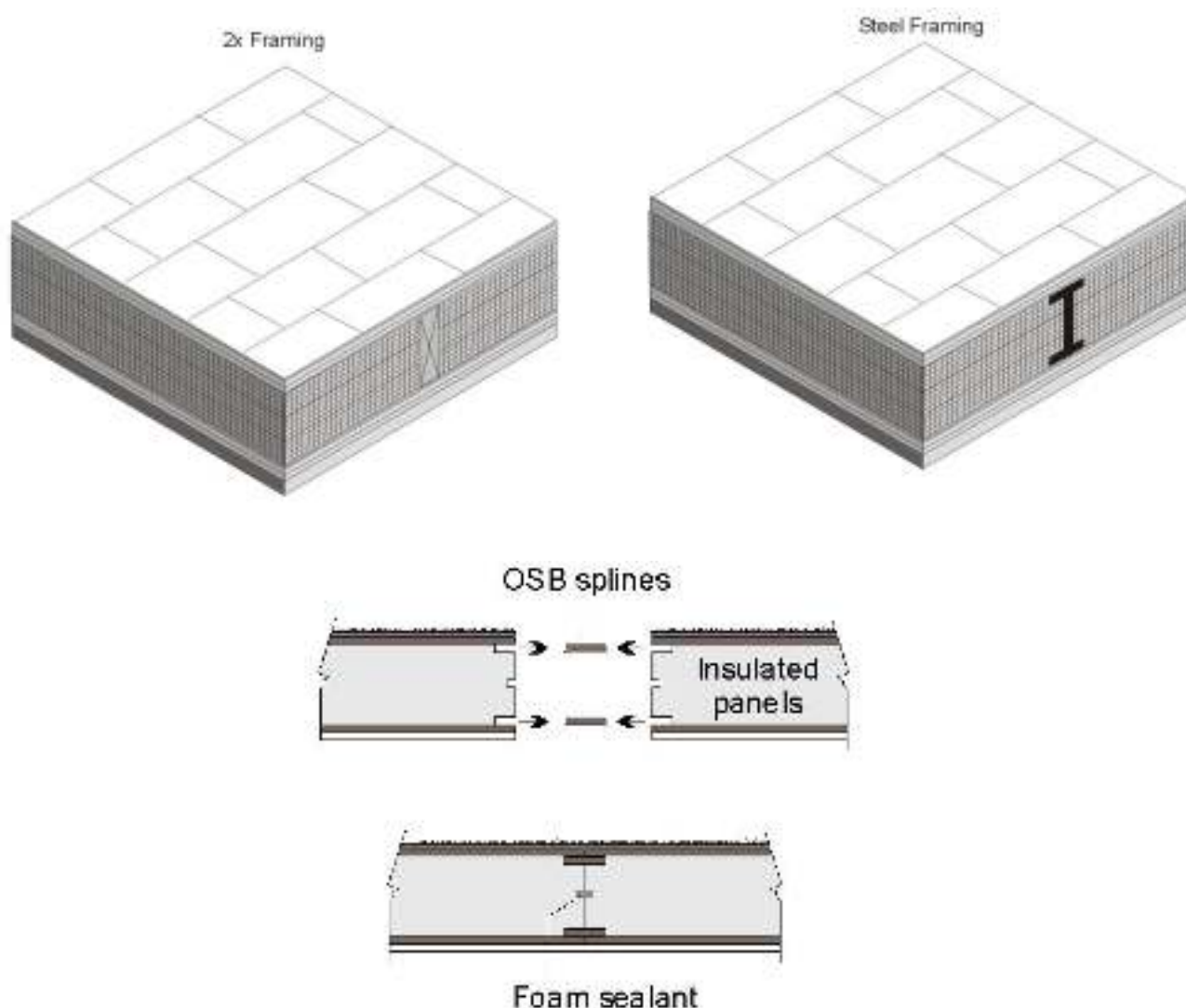
Figure 4.2.3 – SIPs Roof/Ceiling
