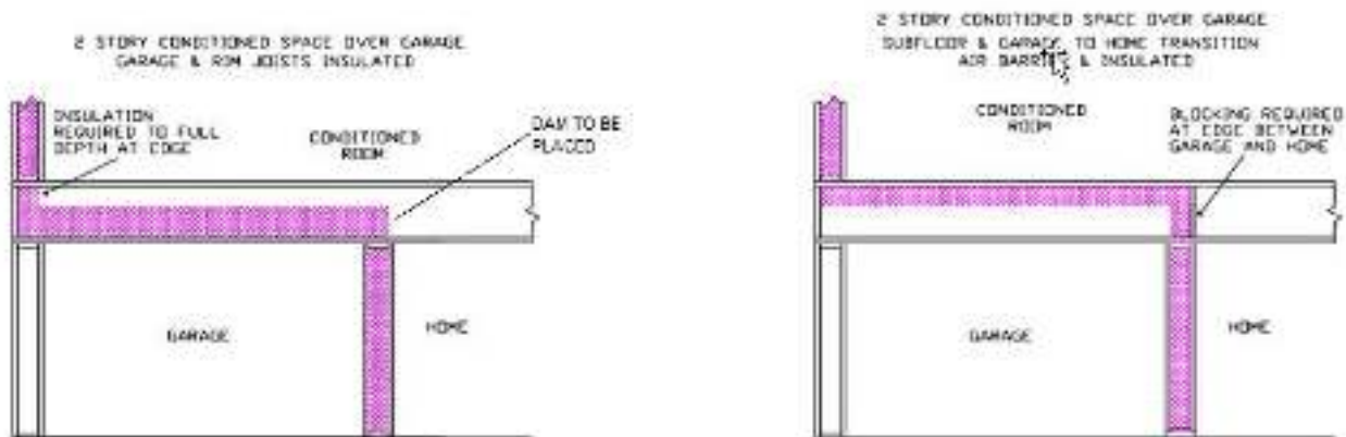
Figure RA3.5-7 Homes with Conditioned Space Over Garage – Spray Polyurethane Foam Insulation
