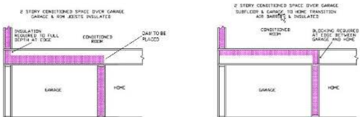
Figure RA3.5-3 Homes with Conditioned Space Over Garage – Loose Fill Insulation
